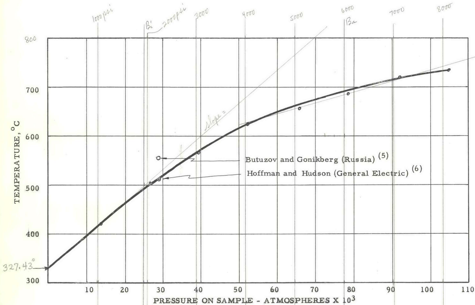
Fig. 5. - Fusion curve of lead
